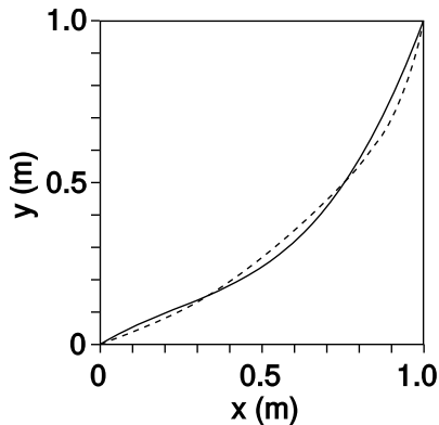
a / Approximations to the brachistochrone curve using a third-order polynomial (solid line), and a seventh-order polynomial (dashed). The latter only improves the time by four milliseconds.
